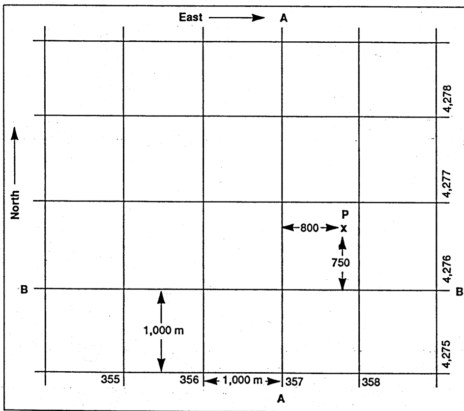
Figure 2. The grid value of line A-A is 357,000 meters east. The grid value of line B-B is 4,276,000 meters north. Point P is 800 meters east and 750 meters north of the grid lines; therefore, the grid coordinates of point P are north 4,276,750 and east 357,800.
